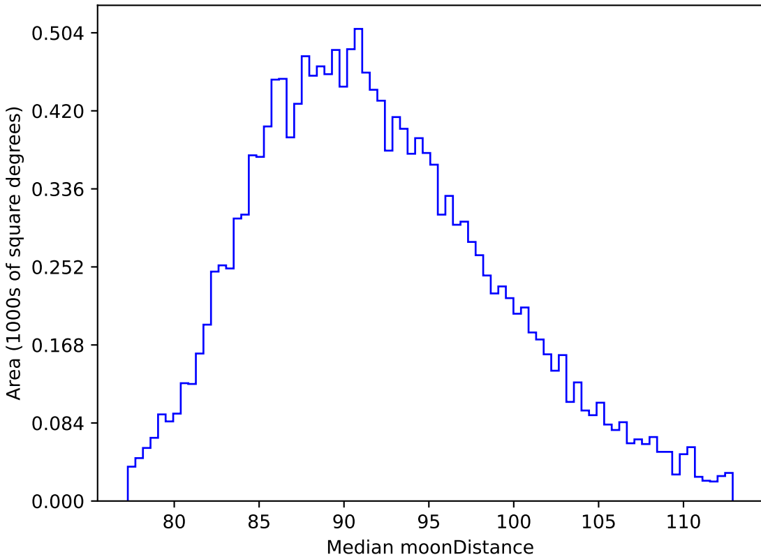
too_10_1v3.4_10yrs WFD i band: Median moonDistance
