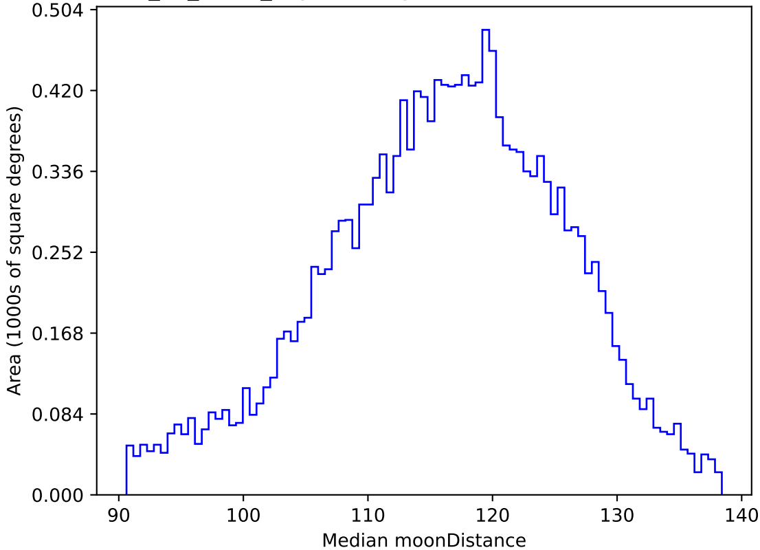
too_10_1v3.4_10yrs WFD g band: Median moonDistance
