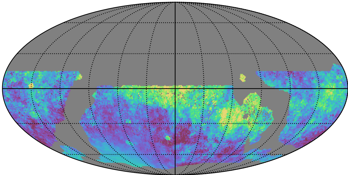
too_10_1v3.4_10yrs WFD all bands: Median moonDistance
