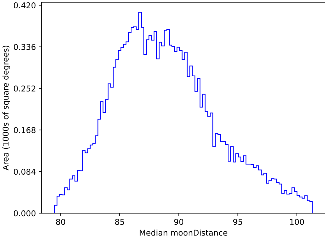
too_10_1v3.4_10yrs WFD all bands: Median moonDistance
