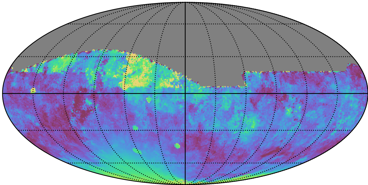
too_10_1v3.4_10yrs All sky z band: Median moonDistance
