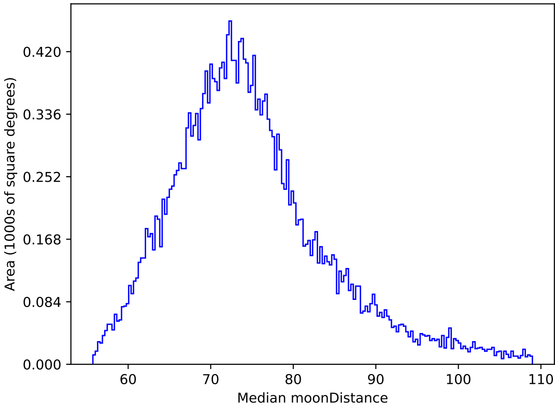
too_10_1v3.4_10yrs All sky z band: Median moonDistance
