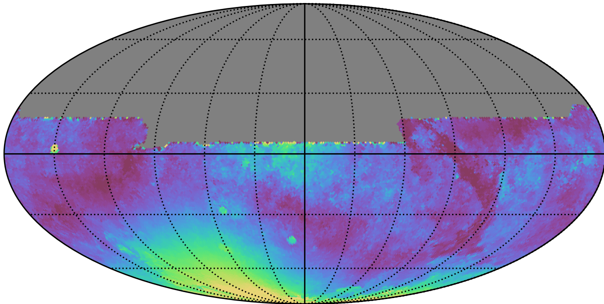
too_10_1v3.4_10yrs All sky y band: Median moonDistance
