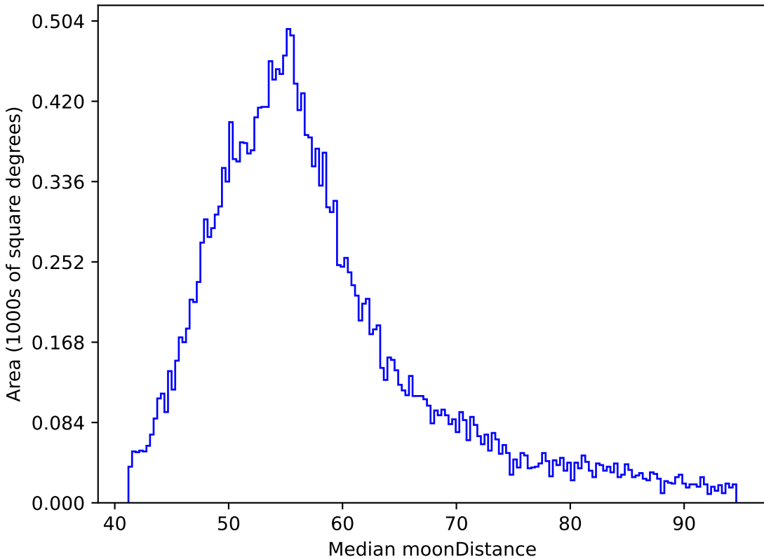
too_10_1v3.4_10yrs All sky y band: Median moonDistance
