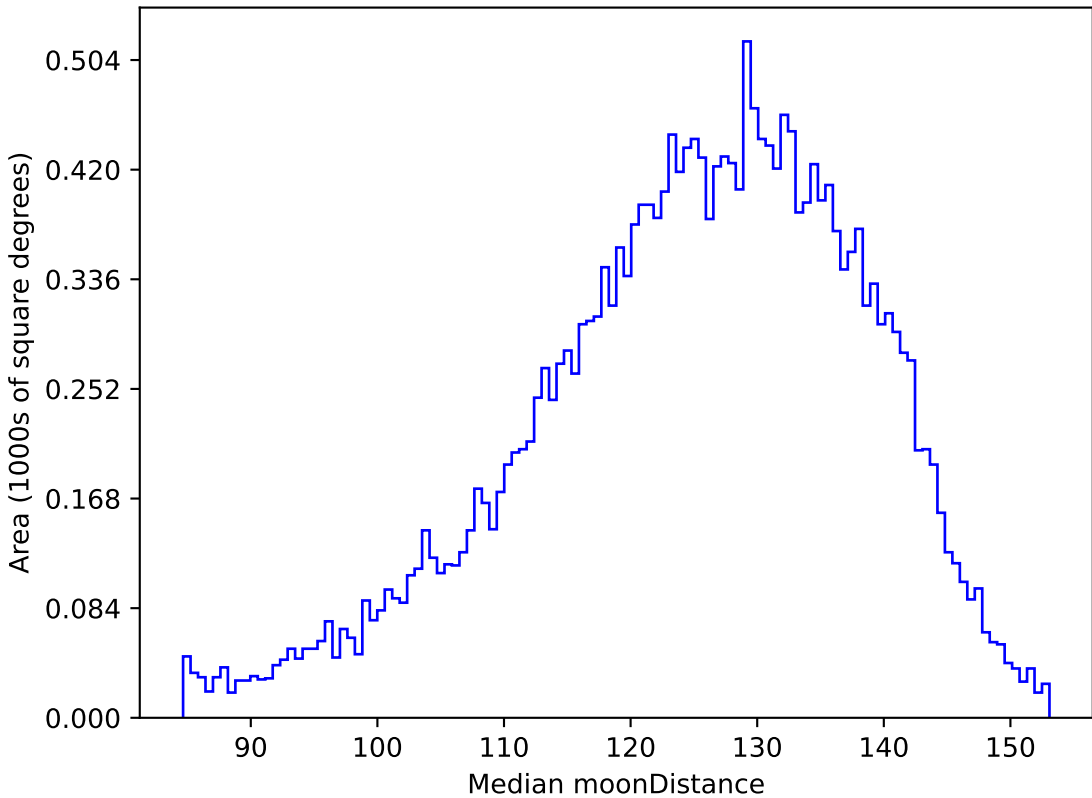
too_10_1v3.4_10yrs All sky u band: Median moonDistance
