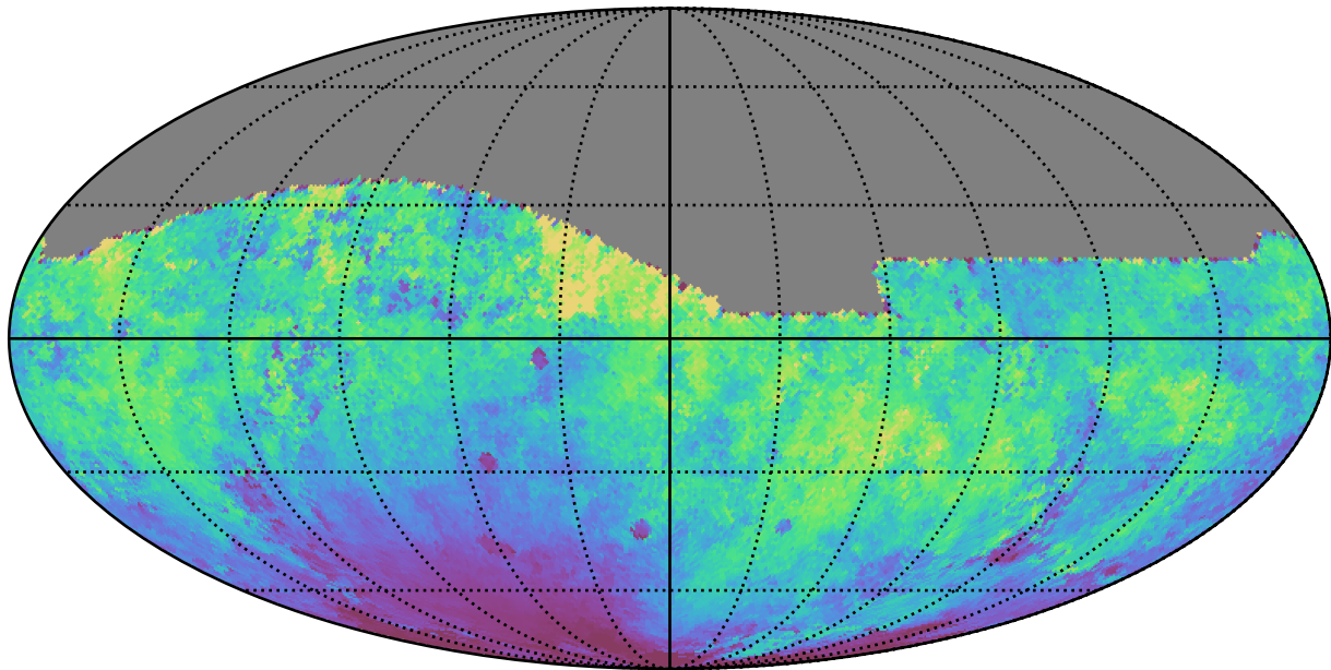
too_10_1v3.4_10yrs All sky r band: Median moonDistance
