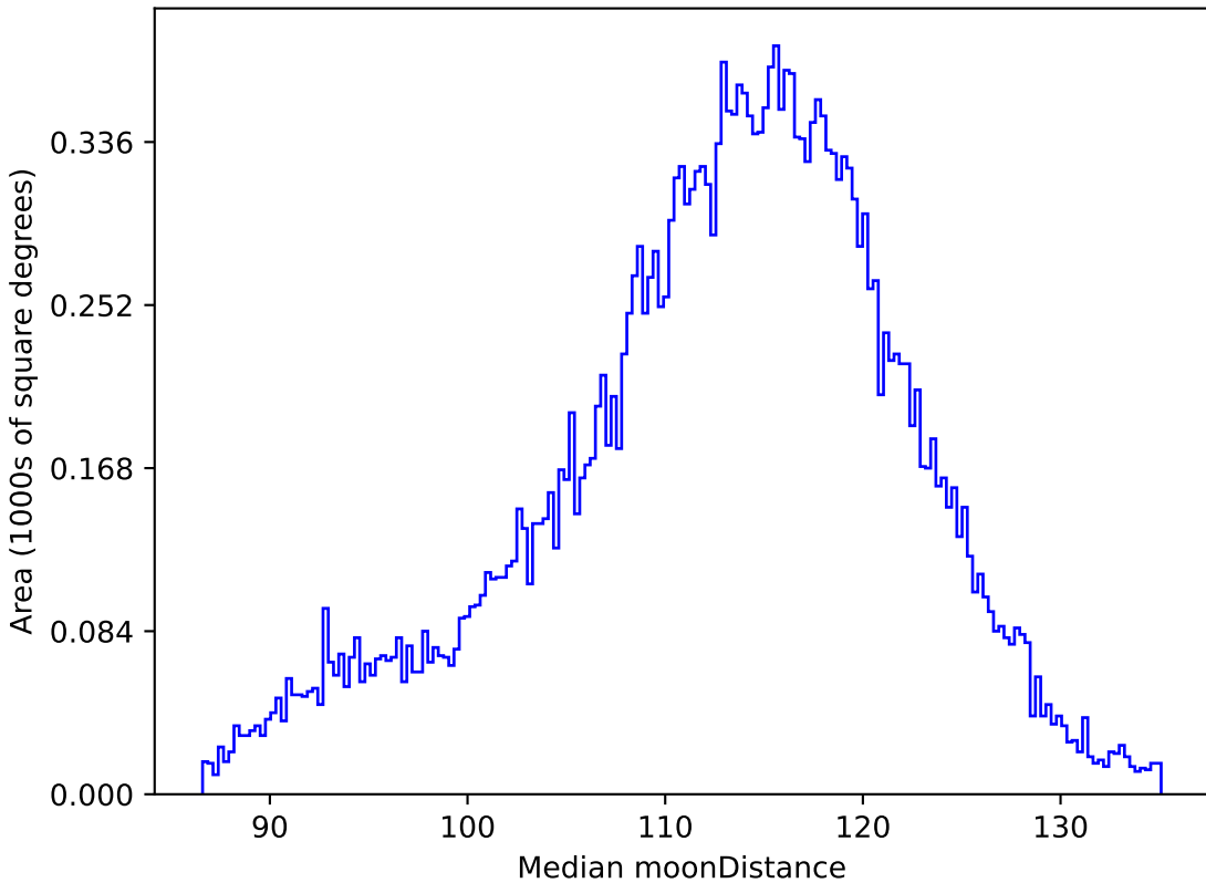
too_10_1v3.4_10yrs All sky r band: Median moonDistance
