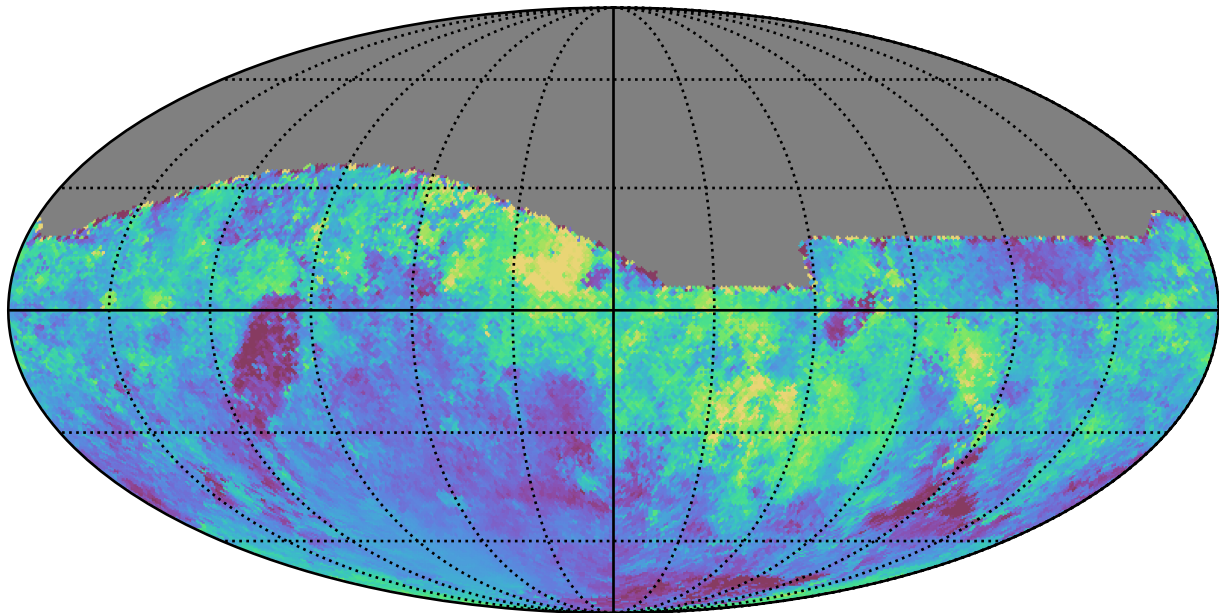
too_10_1v3.4_10yrs All sky i band: Median moonDistance
