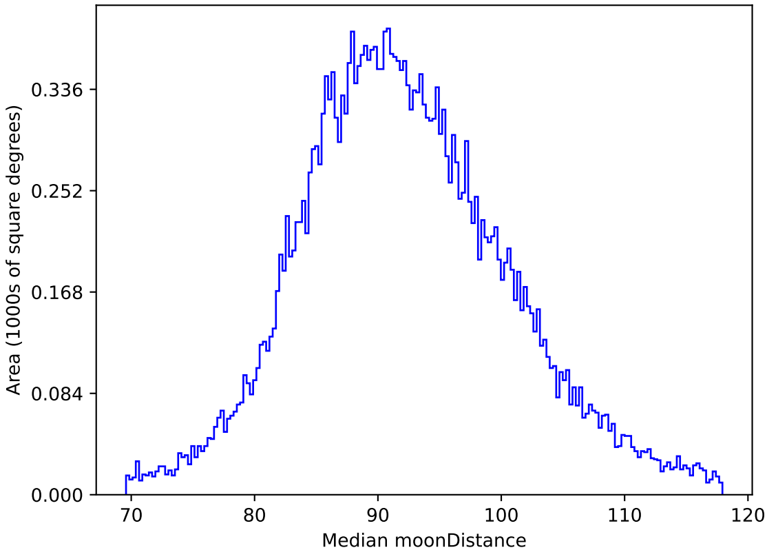
too_10_1v3.4_10yrs All sky i band: Median moonDistance
