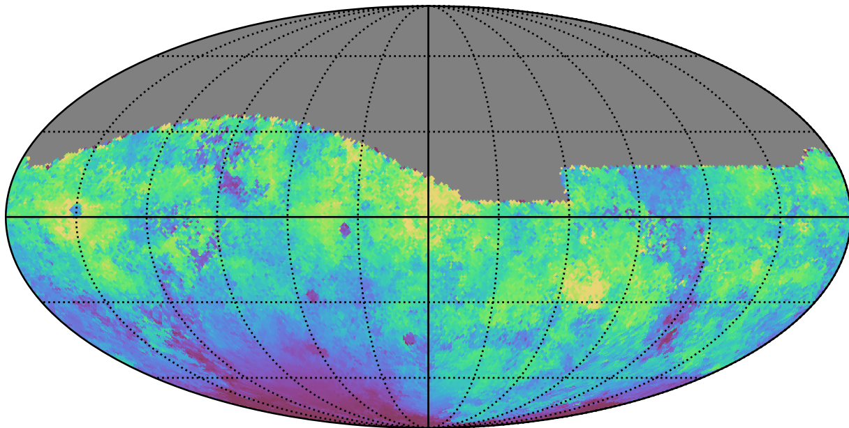
too_10_1v3.4_10yrs All sky g band: Median moonDistance
