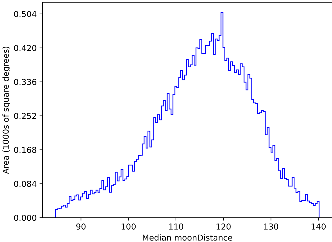
too_10_1v3.4_10yrs All sky g band: Median moonDistance
