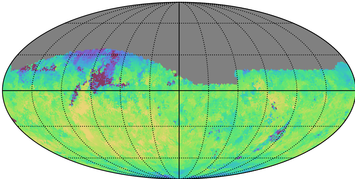
too_10_1v3.4_10yrs Yr 1 z band: Median fiveSigmaDepth
