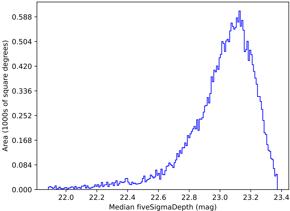
too_10_1v3.4_10yrs Yr 1 z band: Median fiveSigmaDepth
