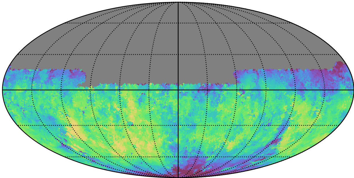
too_10_1v3.4_10yrs Yr 1 y band: Median fiveSigmaDepth
