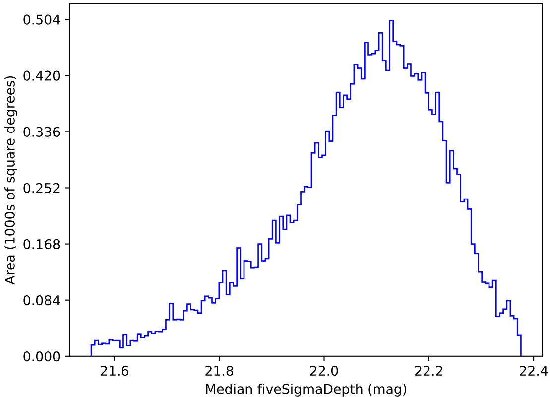
too_10_1v3.4_10yrs Yr 1 y band: Median fiveSigmaDepth
