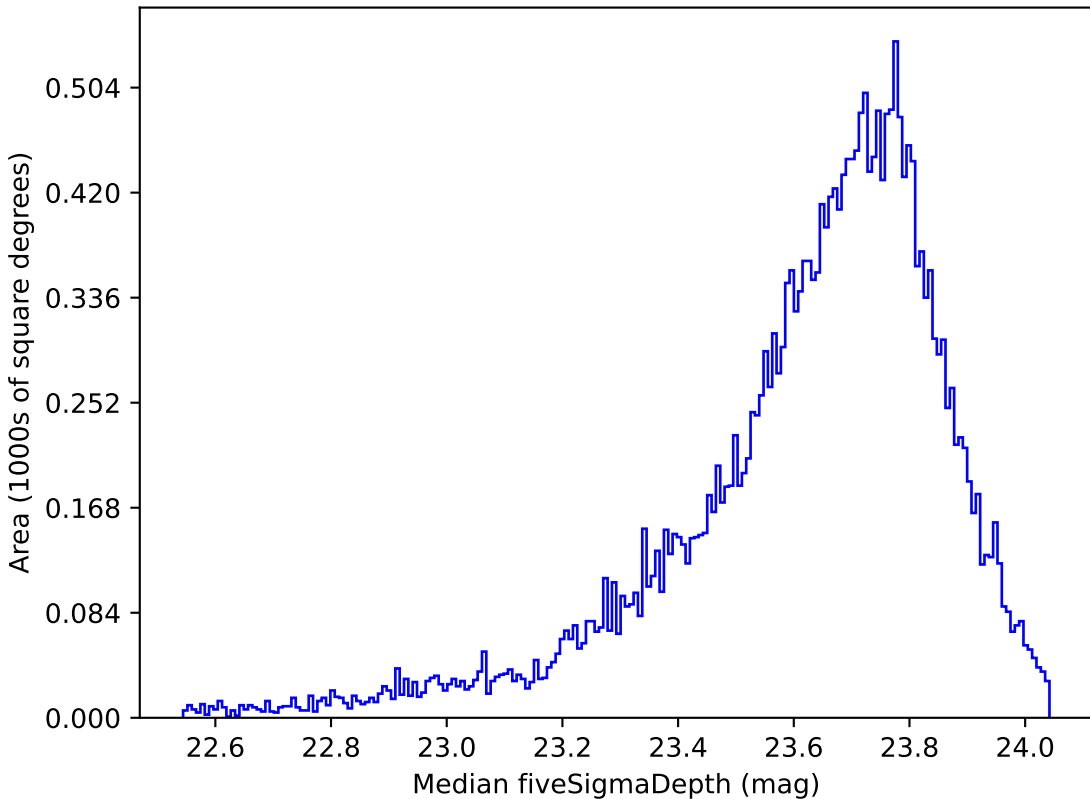
too_10_1v3.4_10yrs Yr 1 i band: Median fiveSigmaDepth
