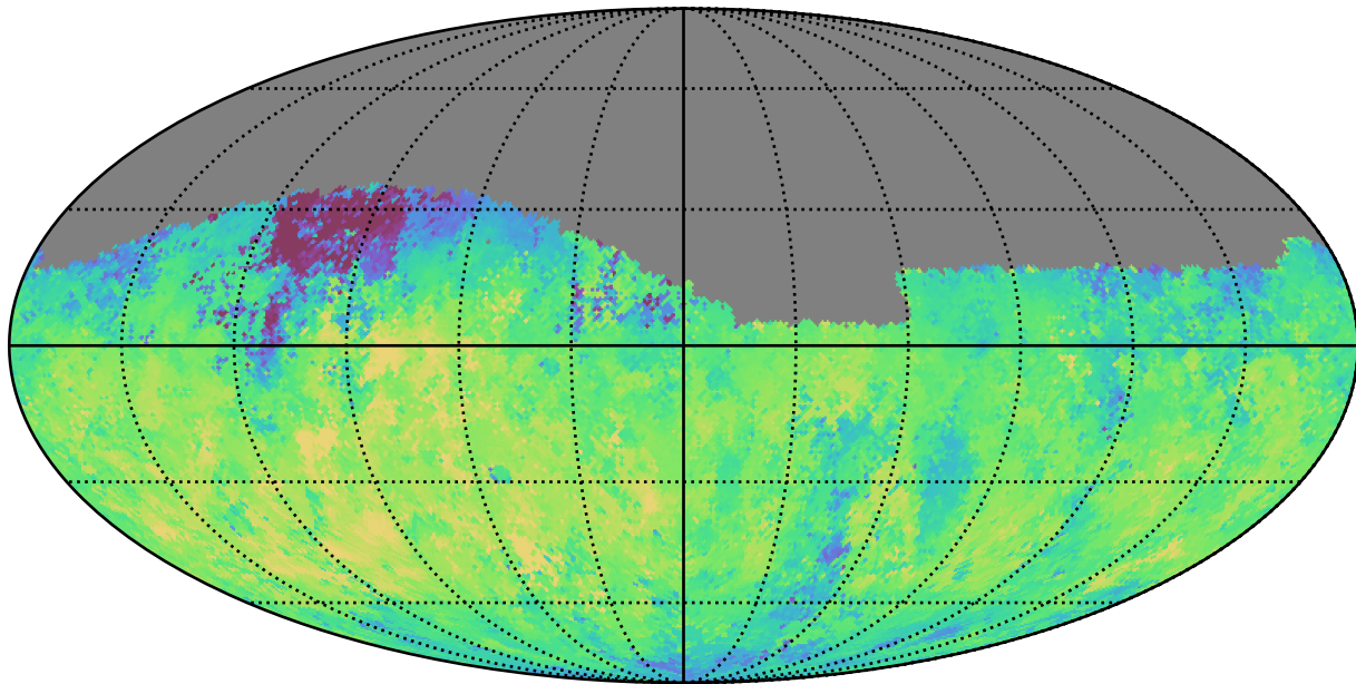
too_10_1v3.4_10yrs Yr 1 g band: Median fiveSigmaDepth
