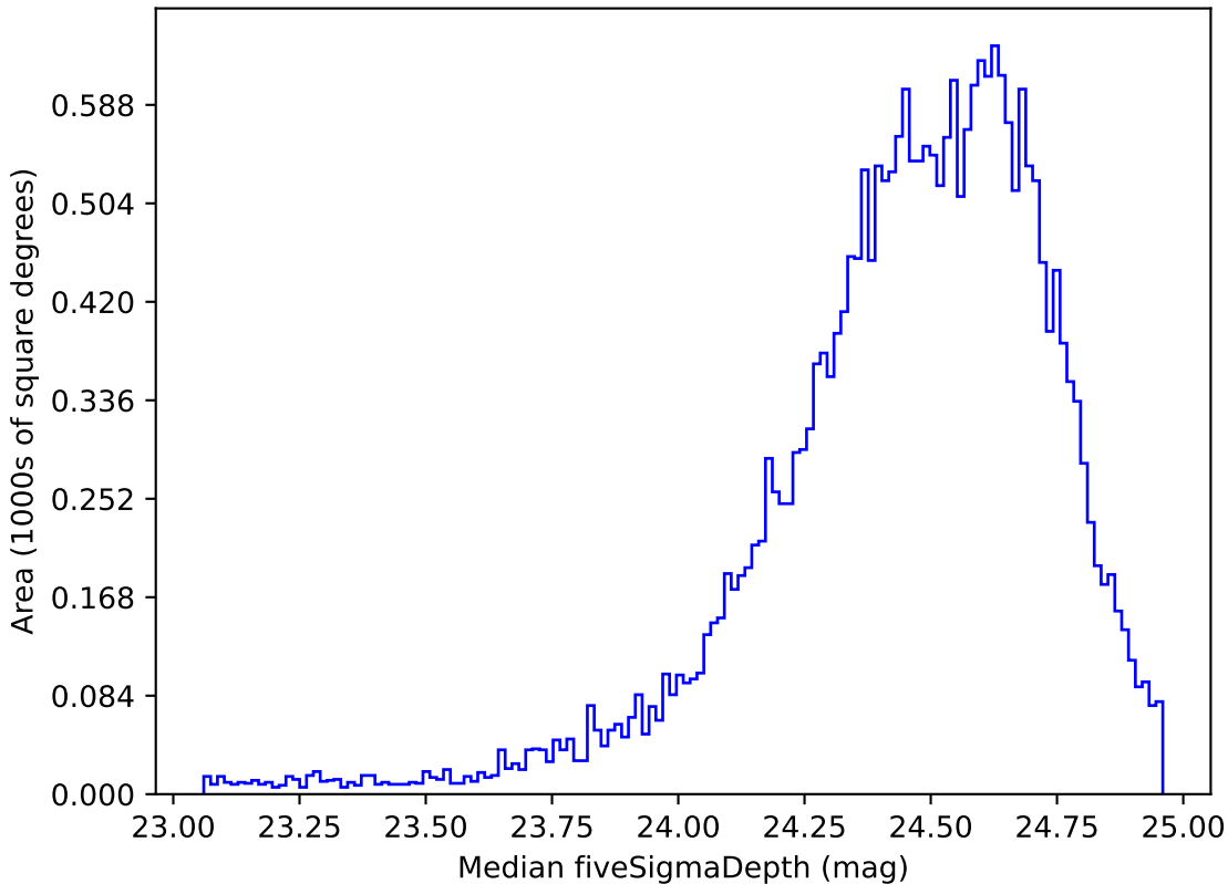
too_10_1v3.4_10yrs Yr 1 g band: Median fiveSigmaDepth
