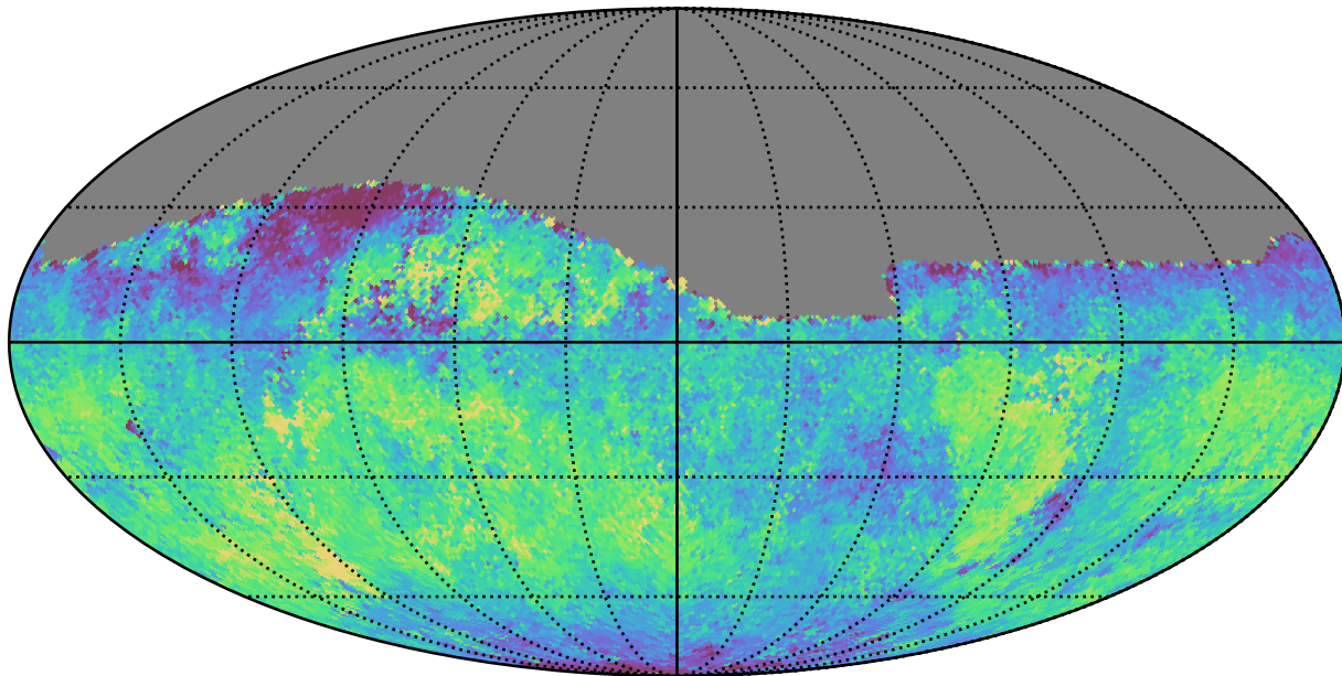
too_10_1v3.4_10yrs Yr 1 all bands: Median fiveSigmaDepth
