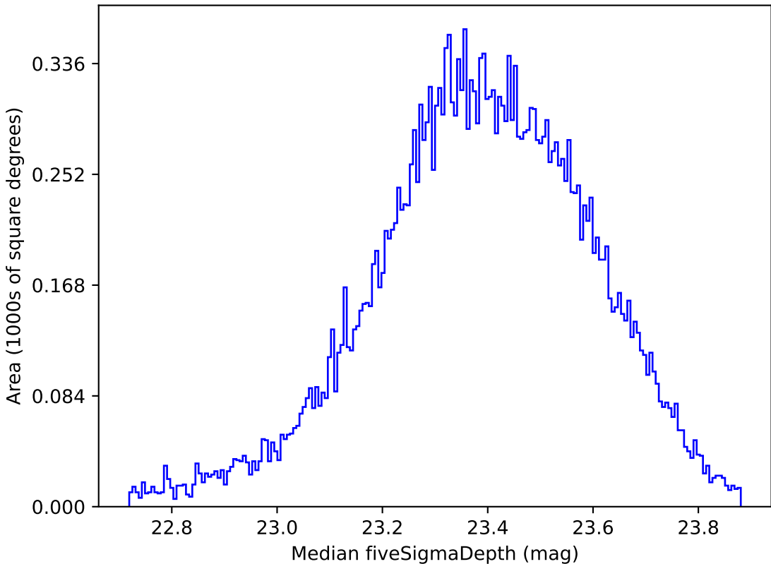
too_10_1v3.4_10yrs Yr 1 all bands: Median fiveSigmaDepth
