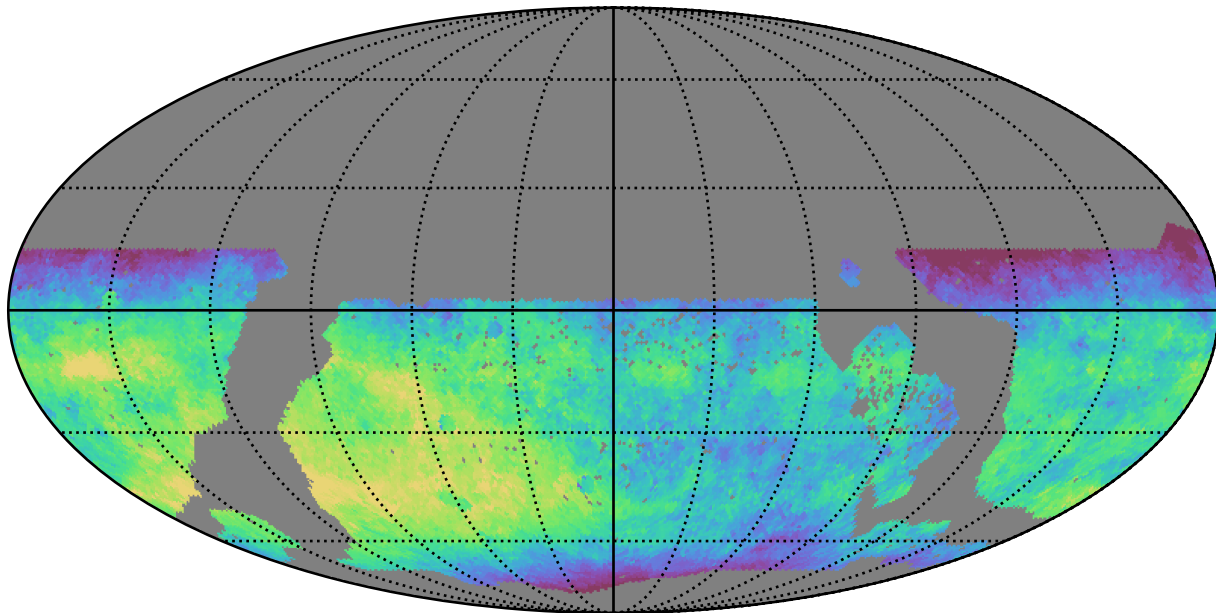
too_10_1v3.4_10yrs WFD z band: Median fiveSigmaDepth
