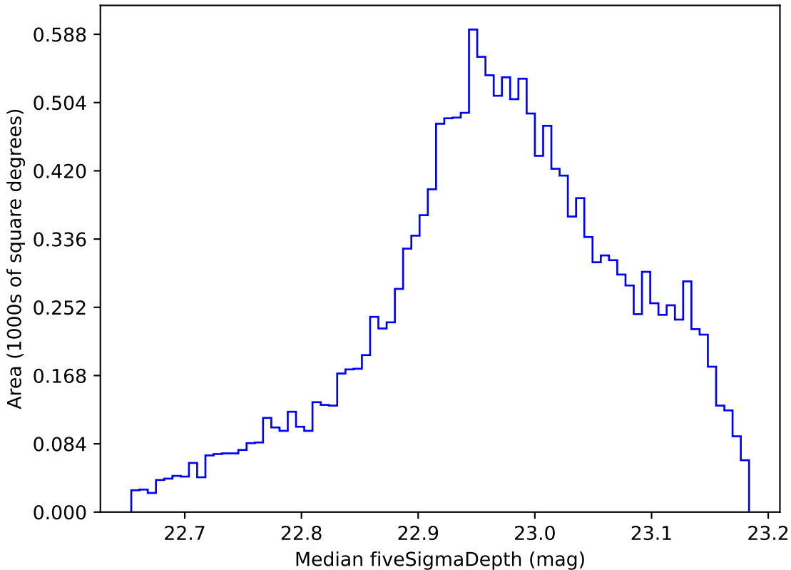
too_10_1v3.4_10yrs WFD z band: Median fiveSigmaDepth
