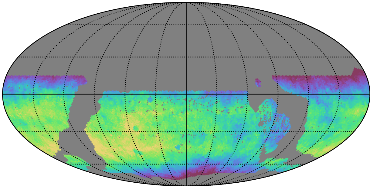
too_10_1v3.4_10yrs WFD y band: Median fiveSigmaDepth
