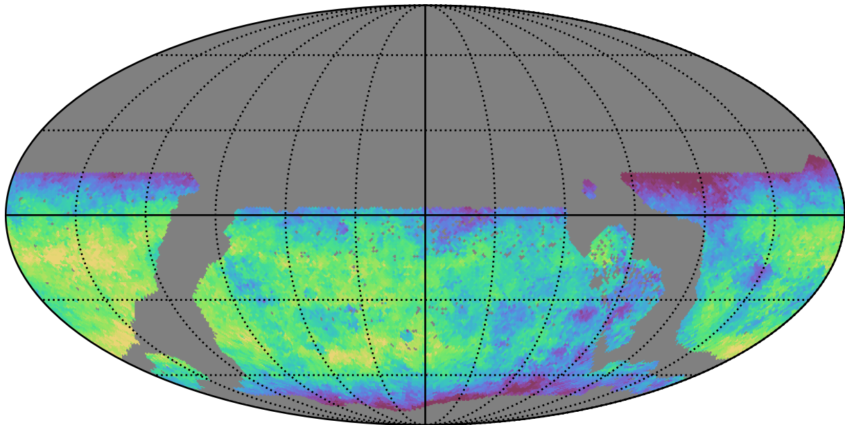
too_10_1v3.4_10yrs WFD u band: Median fiveSigmaDepth
