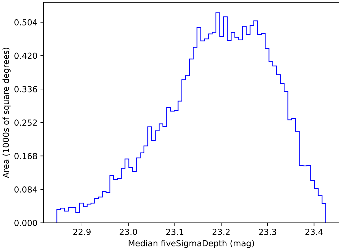
too_10_1v3.4_10yrs WFD u band: Median fiveSigmaDepth
