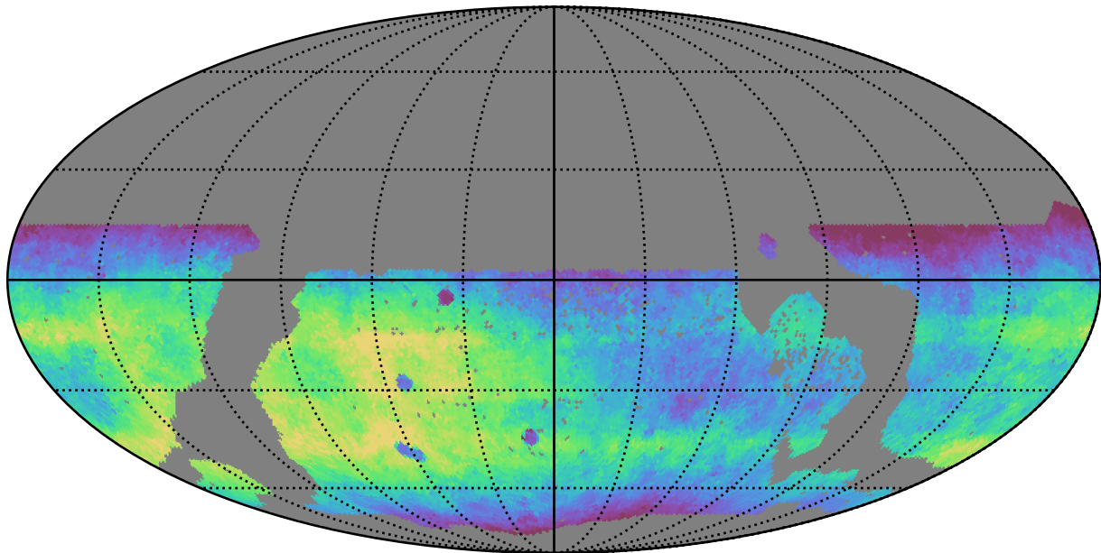
too_10_1v3.4_10yrs WFD r band: Median fiveSigmaDepth
