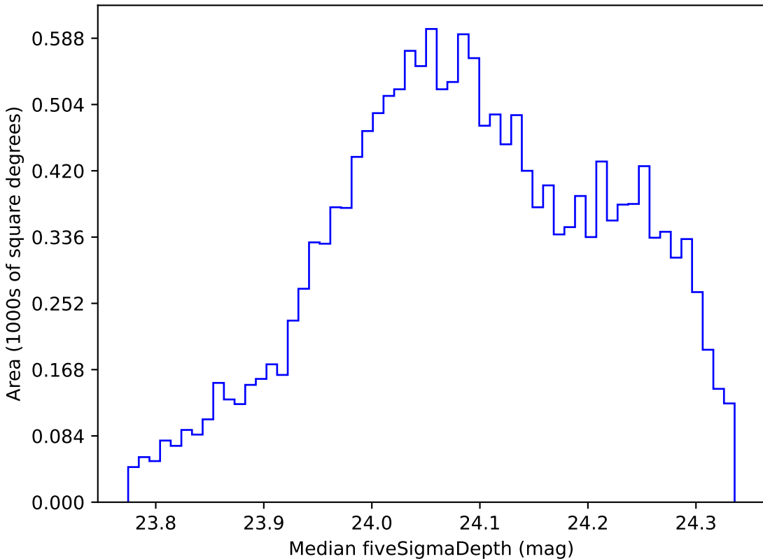
too_10_1v3.4_10yrs WFD r band: Median fiveSigmaDepth
