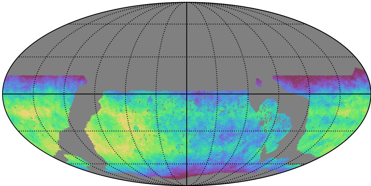
too_10_1v3.4_10yrs WFD i band: Median fiveSigmaDepth
