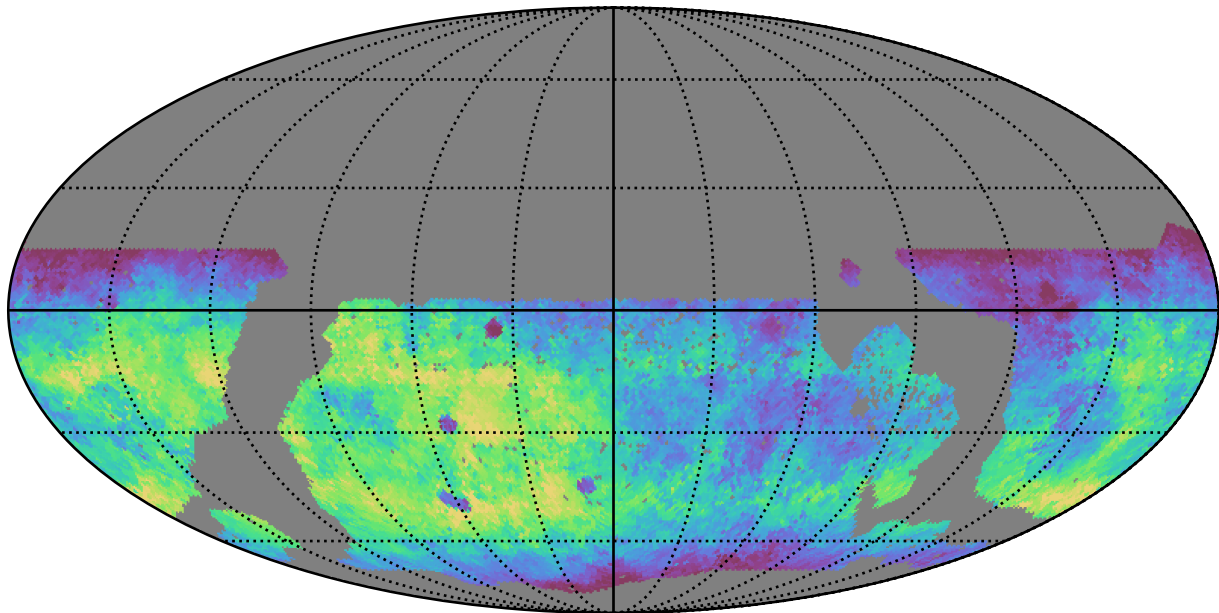
too_10_1v3.4_10yrs WFD g band: Median fiveSigmaDepth
