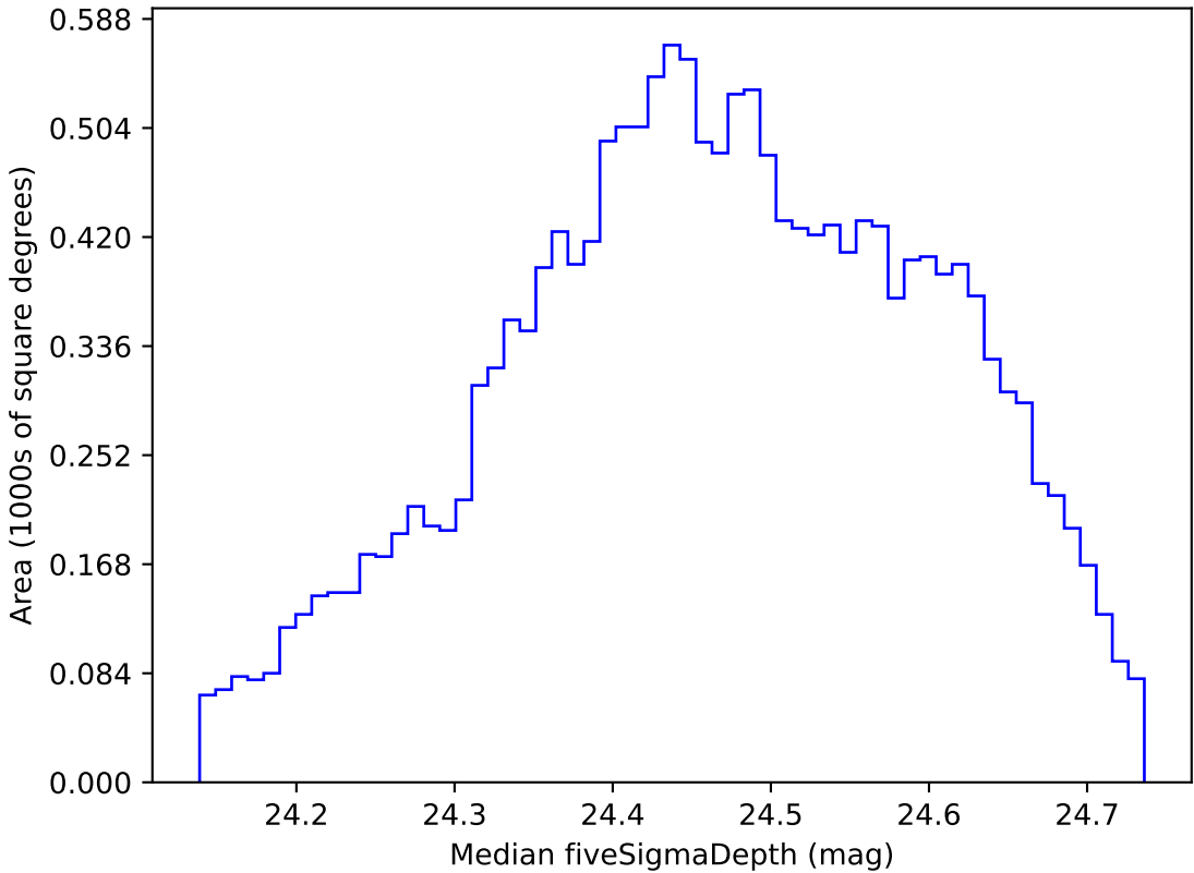
too_10_1v3.4_10yrs WFD g band: Median fiveSigmaDepth
