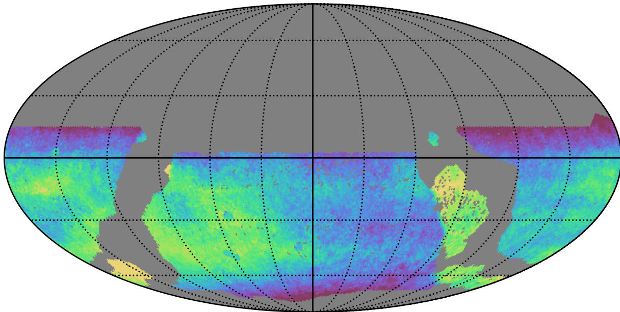
too_10_1v3.4_10yrs WFD all bands: Median fiveSigmaDepth
