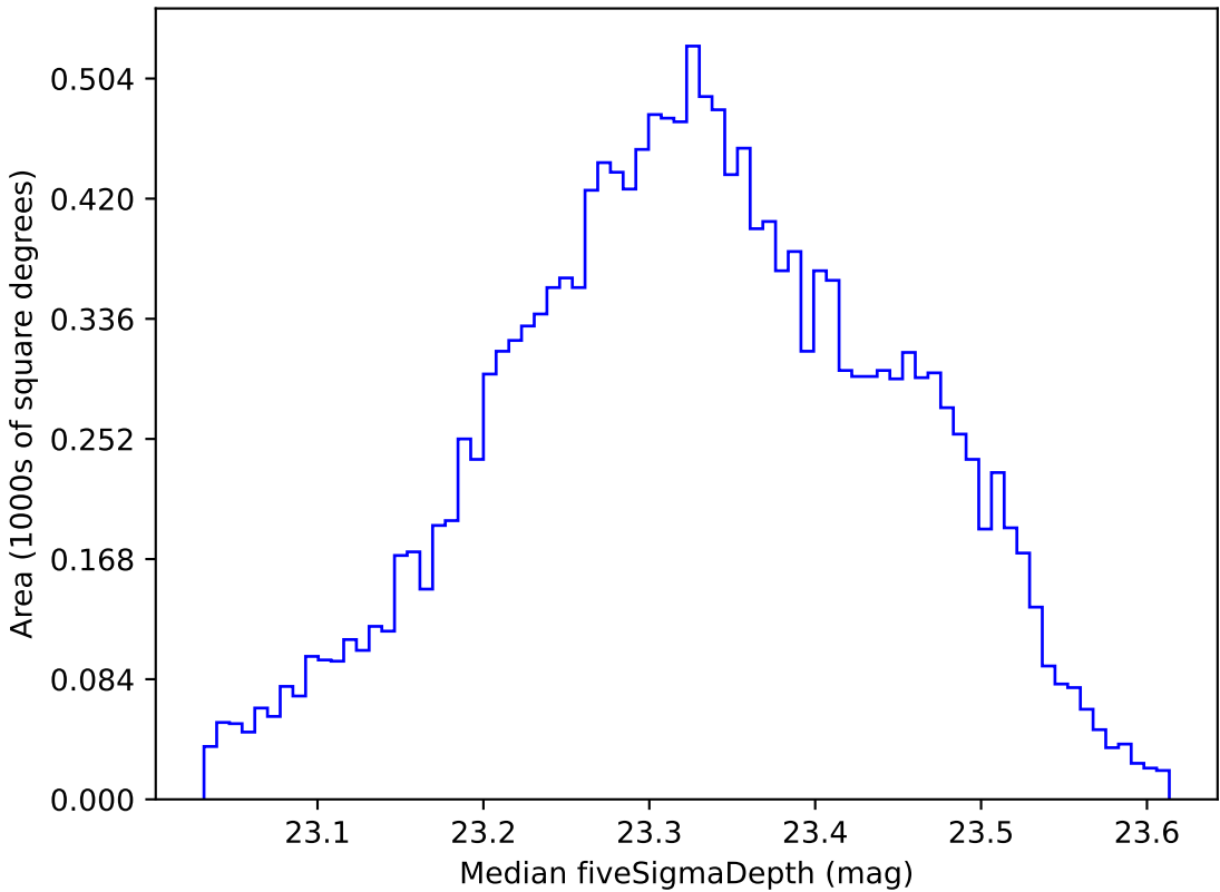
too_10_1v3.4_10yrs WFD all bands: Median fiveSigmaDepth
