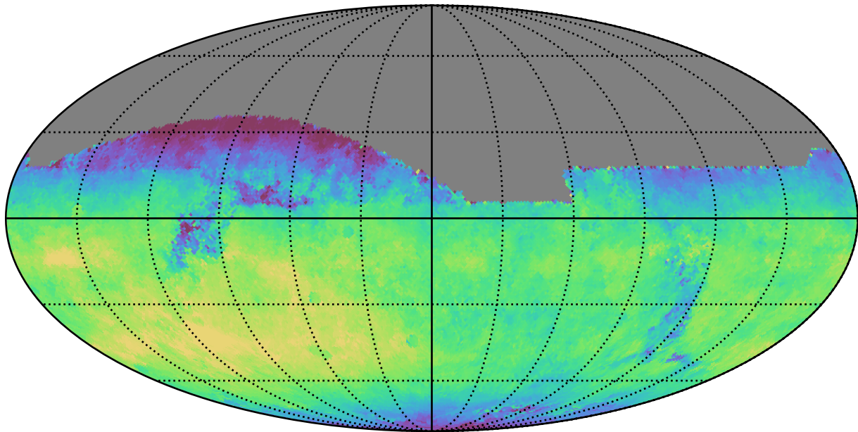
too_10_1v3.4_10yrs All sky z band: Median fiveSigmaDepth
