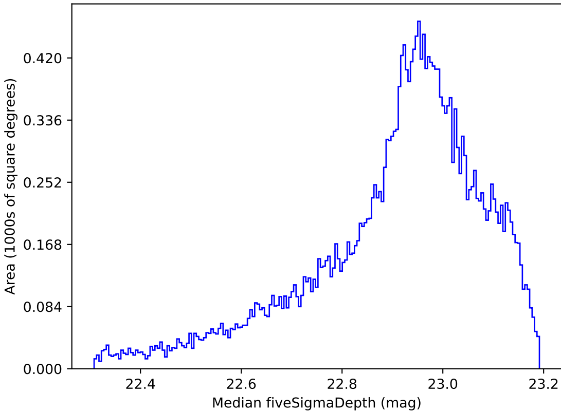
too_10_1v3.4_10yrs All sky z band: Median fiveSigmaDepth
