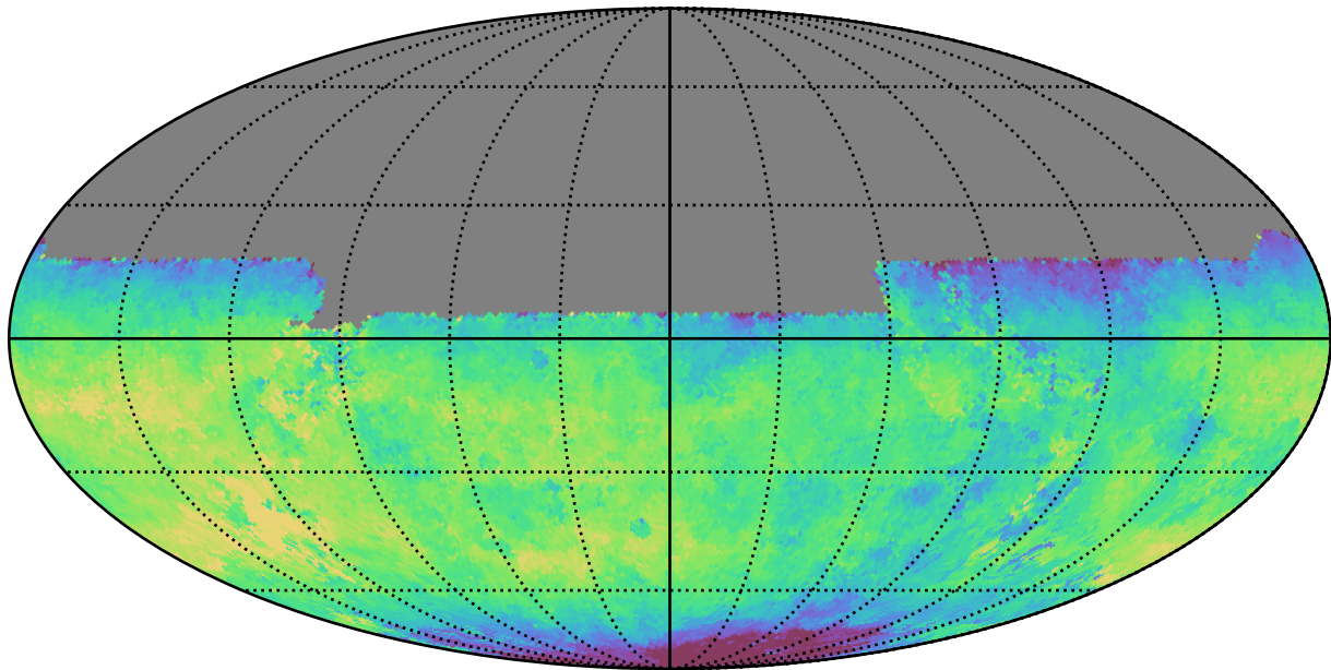
too_10_1v3.4_10yrs All sky u band: Median fiveSigmaDepth
