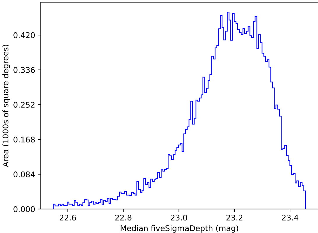
too_10_1v3.4_10yrs All sky u band: Median fiveSigmaDepth
