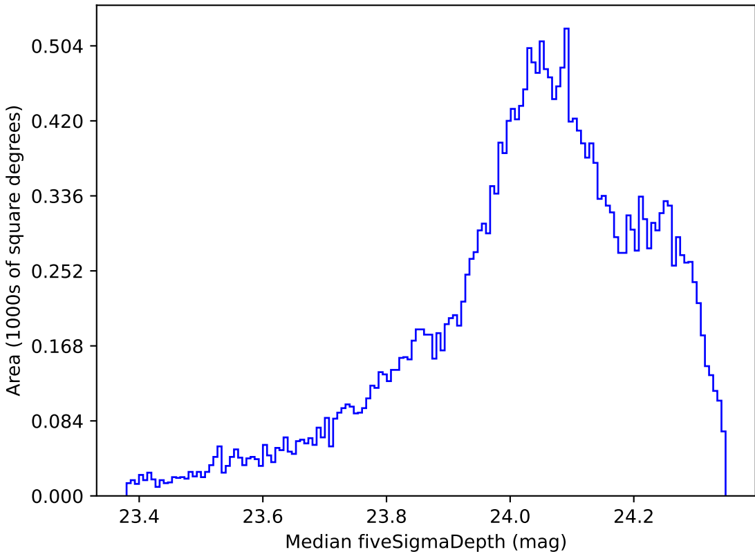
too_10_1v3.4_10yrs All sky r band: Median fiveSigmaDepth
