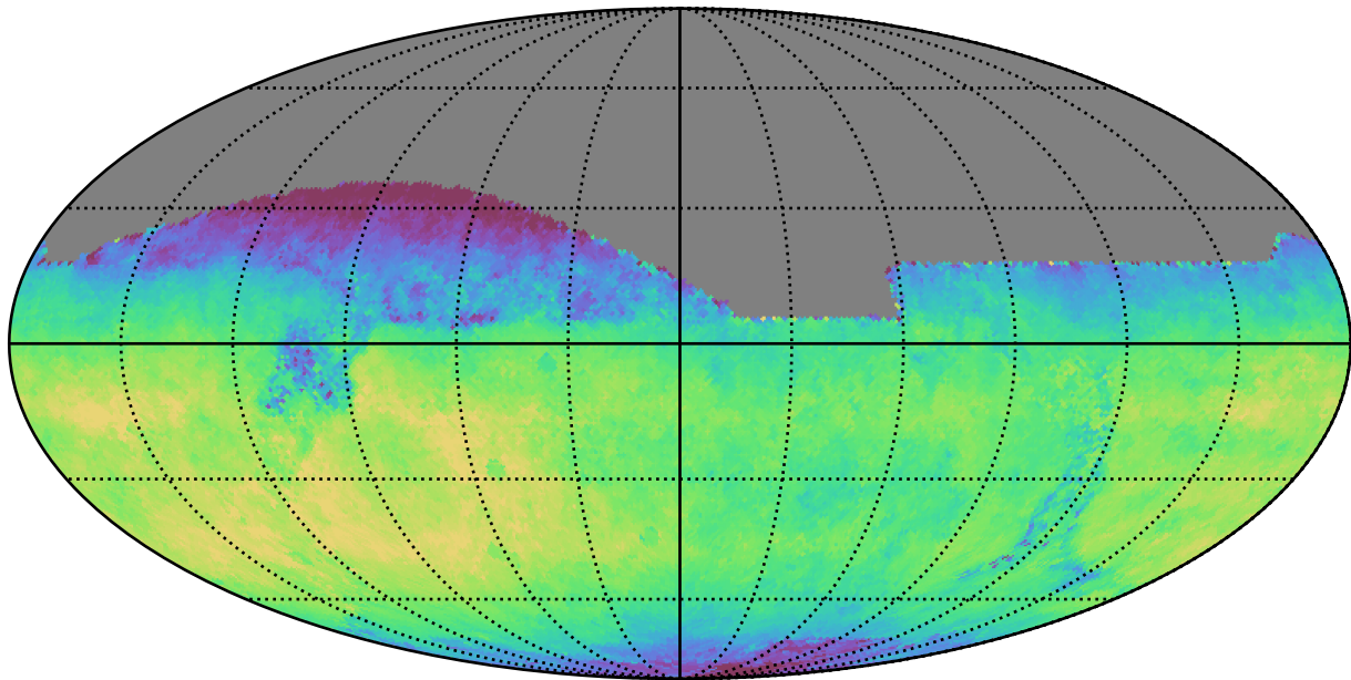
too_10_1v3.4_10yrs All sky i band: Median fiveSigmaDepth
