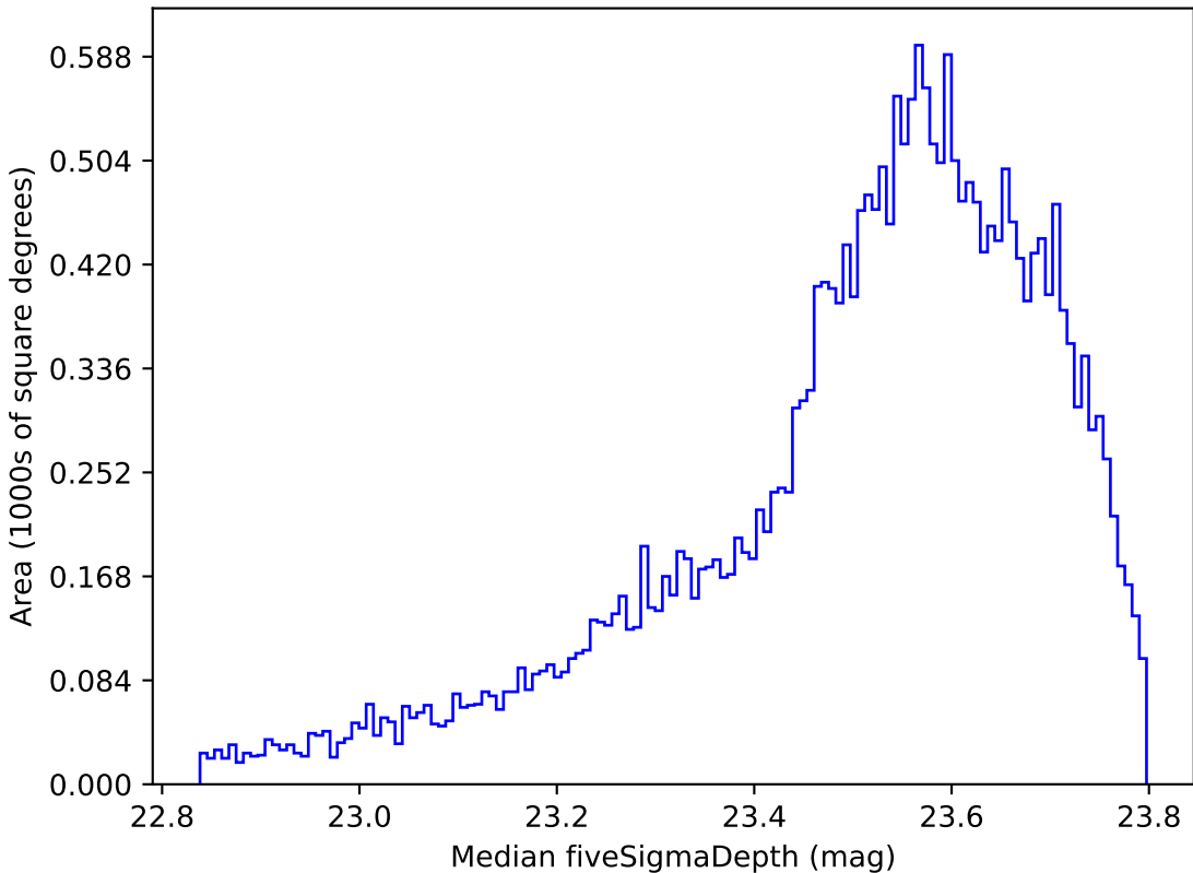
too_10_1v3.4_10yrs All sky i band: Median fiveSigmaDepth
