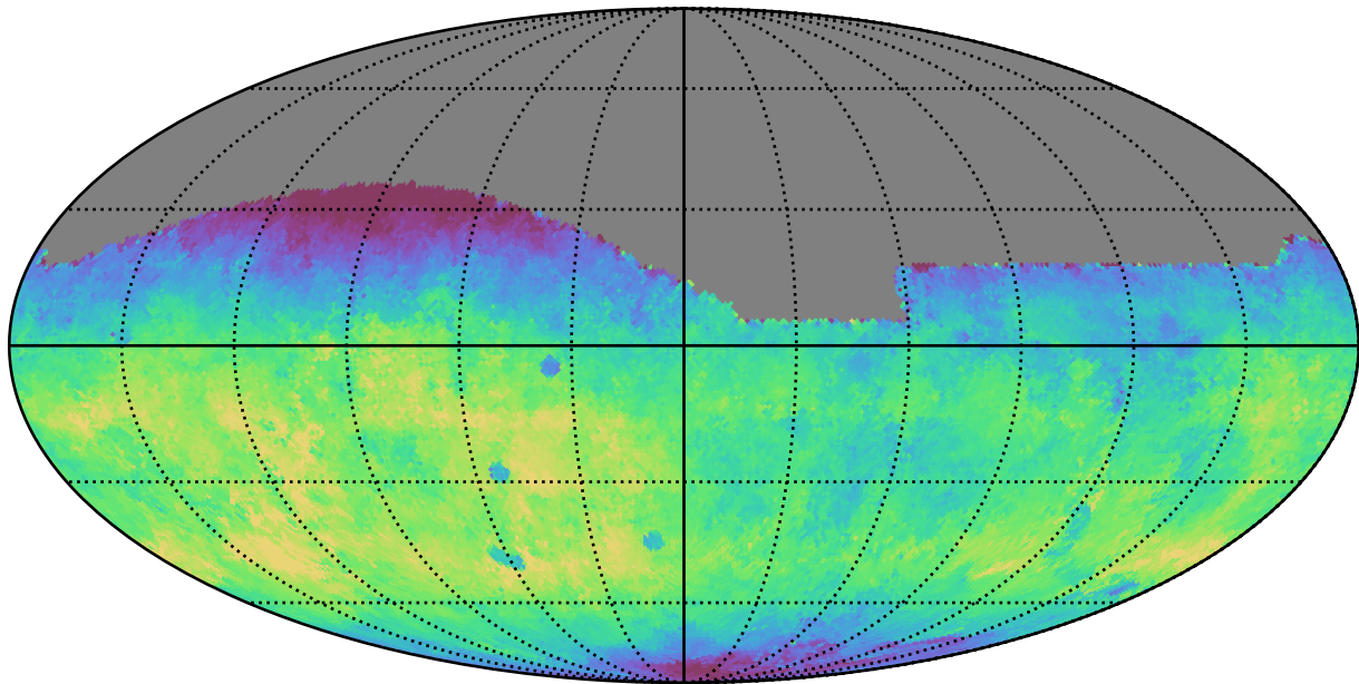
too_10_1v3.4_10yrs All sky g band: Median fiveSigmaDepth
