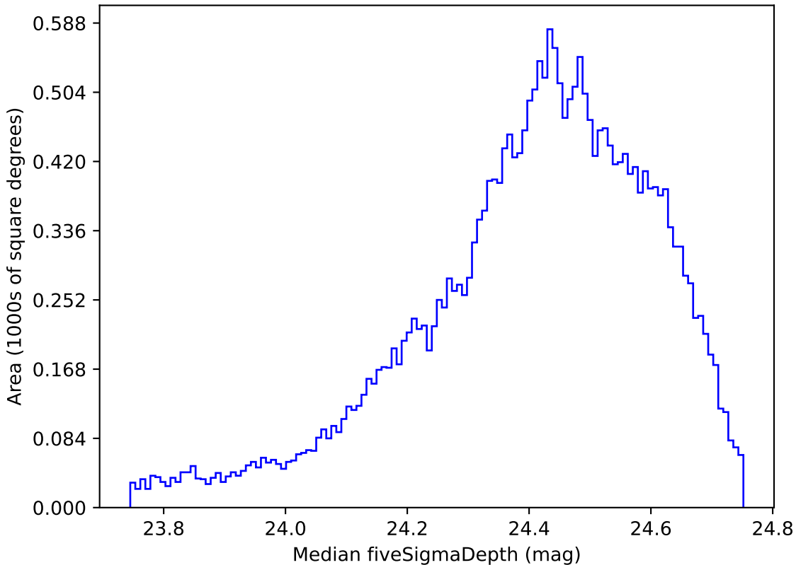
too_10_1v3.4_10yrs All sky g band: Median fiveSigmaDepth
