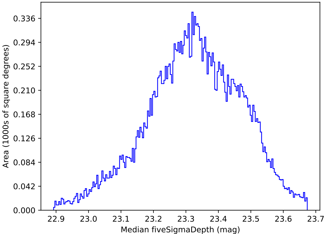
too_10_1v3.4_10yrs All sky all bands: Median fiveSigmaDepth
