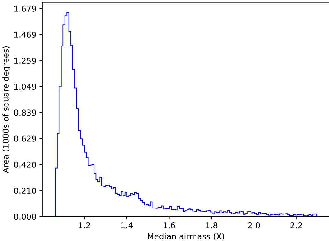
too_10_1v3.4_10yrs Yr 1 z band: Median airmass
