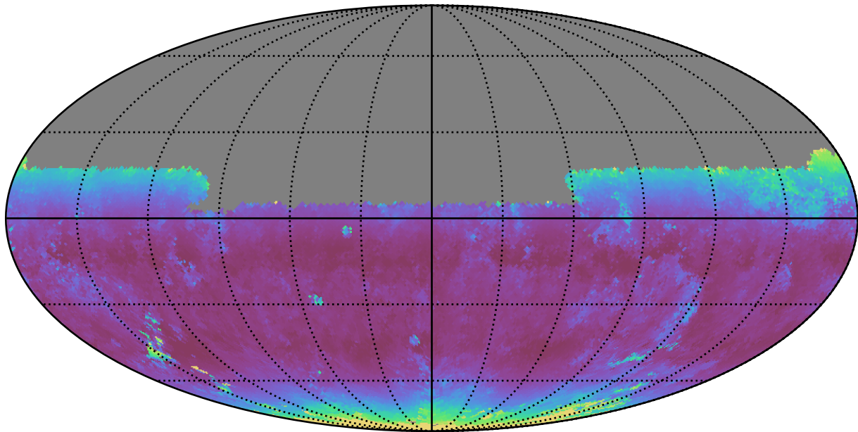
too_10_1v3.4_10yrs Yr 1 y band: Median airmass
