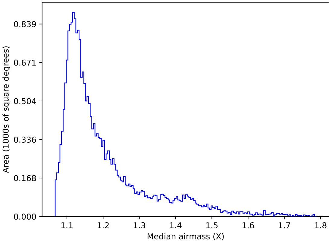
too_10_1v3.4_10yrs Yr 1 y band: Median airmass
