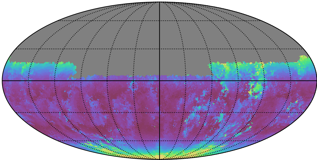
too_10_1v3.4_10yrs Yr 1 u band: Median airmass
